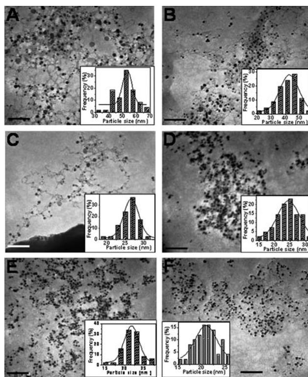
Fig. 2 Representative TEM images of the gold nanoparticles synthesized at 20 °C (A), 30 °C (B), 40 °C (C), 50 °C (D), 60 °C (E) and 70 °C (F). Scale bar presented in TEM images (A–F) is 200 nm. Insets show particle size distributions of gold nanoparticles at different temperatures. Different bin sizes were used to obtain information on the size distribution of the particles appropriate to the samples investigated.
