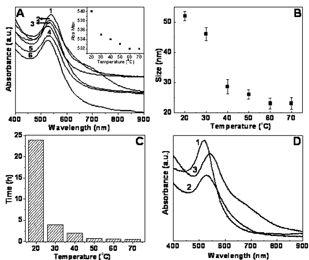
Fig. 1 (A) Representative UV-vis spectra of gold nanoparticles synthesized using cefaclor at 20 °C (curve 1), 30 °C (curve 2), 40 °C (curve 3), 50 °C (curve 4), 60 °C (curve 5) and 70 °C (curve 6). Inset shows the absorbance maxima of curves 1–6 vs. temperature. The absorption maxima of the gold nanoparticle spectra were determined after spectra were smoothed (11 point adjacent averaging) and the derivative spectra obtained (Origin software). (B) DLS data, the size of gold nanoparticles versus temperature. (C) Maximum time for the complete reduction of gold ions using cefaclor at different temperatures. (D) UV-vis spectra of gold nanoparticles synthesized using \text{NaBH}_4 (curve 1), after binding of cefaclor to \text{NaBH}_4 reduced gold nanoparticles (curve 2) and the gold nanoparticles synthesized using cefaclor at 20 °C (curve 3).
