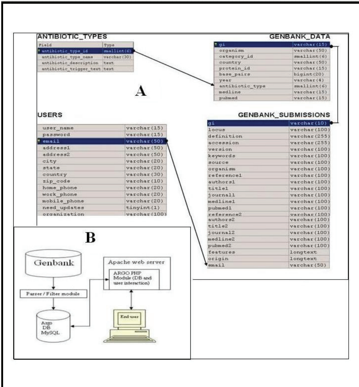
Figure 1: A representation of ARGO (A: database schema, B: database architecture). The relationships in the database are shown in the schema using connecting lines (arrow-heads indicate many and solid-balls indicate one )
