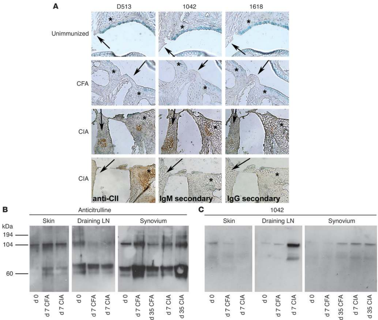
Figure 5 D513, 1042, and 1618 monoclonal antibodies bind antigens within the inflamed synovium of mice with CIA. (A) Immunohistochemistry was performed using 4 \mu\text{g}/\text{ml} D513, 1042, and 1618. Antibody binding is indicated by DAB precipitate (brown). Tissue was counterstained with methyl green. A mix of anti-CII monoclonal antibodies and secondary reagents without primary antibody served as negative controls for staining the synovium. Representative serial sections are shown. Magnification, \times 100 . Arrows point to synovium, and asterisks indicate cartilage. (B) Skin from the site of immunization, draining inguinal LN, and synovium were collected from unimmunized mice, mice immunized with CFA, or mice with CIA at different time points. Western blots of the protein isolated from these tissues were performed with a polyclonal antibody that recognizes the amino acid citrulline or (C) with the monoclonal antibodies 1042, 1618, and D513. Representative blots are shown. Results of Western blots probed with antibodies 1618 and D513 were essentially identical to 1042 and, thus, are not shown.
