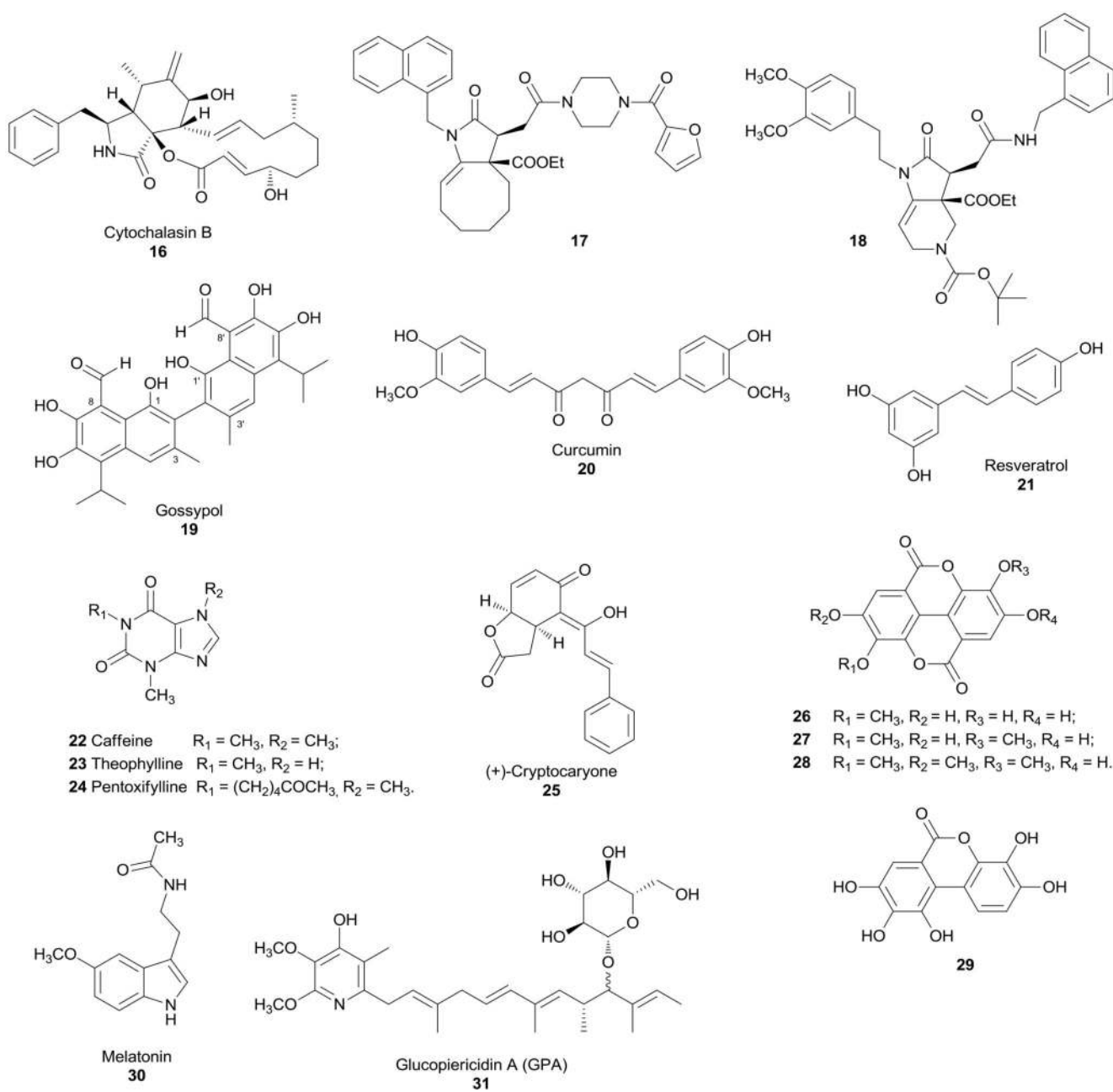
Figure 2. Structures of natural compounds that inhibit GLUTs.
