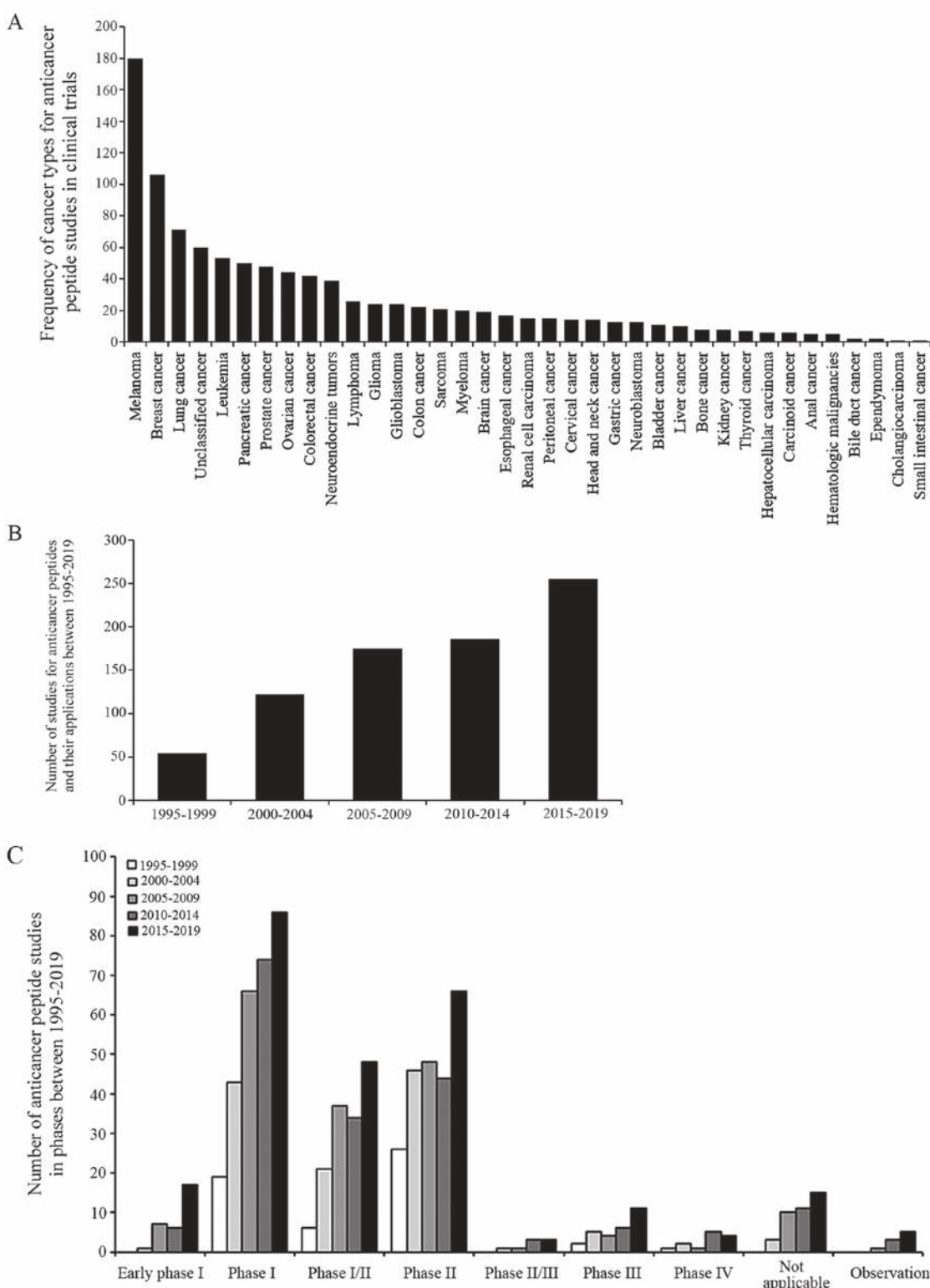
Figure 4. Number of ACP studies for the drug and biological intervention. (A) Frequency of cancer types from 792 ACP studies, which were submitted on the ClinicalTrials.gov website, including 36 cancer types and unclassified cancer types. The unclassified cancer types were reported as solid tumors, cancer or neoplasms. (B) Number of ACP studies in every 5-year period between 1995-2019 was continuously increased. (C) Furthermore, from 1995-2019, >98% of these ACP studies were an intervention study type, including clinical trial in early phase I, phase I, I/II, II, II/III, III, IV and not applicable, while <2% of them were an observation study type, which cannot assign a specific intervention or treatment. Source:www.clinicaltrials.gov search on Feb 4, 2020 with drug, biological and peptide key words in cancer. ACP, anticancer peptide.
