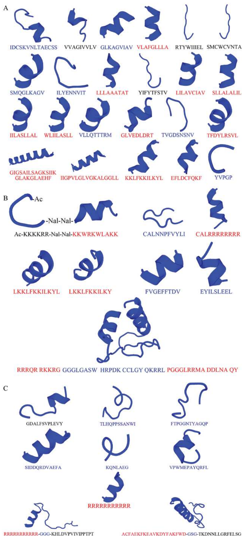
Figure 3. Conformation of anticancer peptides predicted using PEP-FOLD 3.5 ( https://mobyli.rpbs.univ-paris-diderot.fr/cgi-bin/portal.py#forms::PEP-FOLD3 ). (A) Natural, (B) modified and (C) targeting peptides corresponding to Tables II-IV, respectively, performed in three conformations including extend (black alphabet amino acid sequences), coiled (blue alphabet amino acid sequences) and \alpha -helix (red alphabet amino acid sequences).
