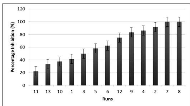
Fig. 1 Inhibition of Calu-3 lung cancer cell attachment upon treatment with agarwood hydrosol tested using Trypan blue dye attachment assay. Samples were prepared based on Central Composite Design (CCD) with two factors (hydrosol amount and exposure duration) at three levels (high, medium, low). Samples (agarwood hydrosol) were
