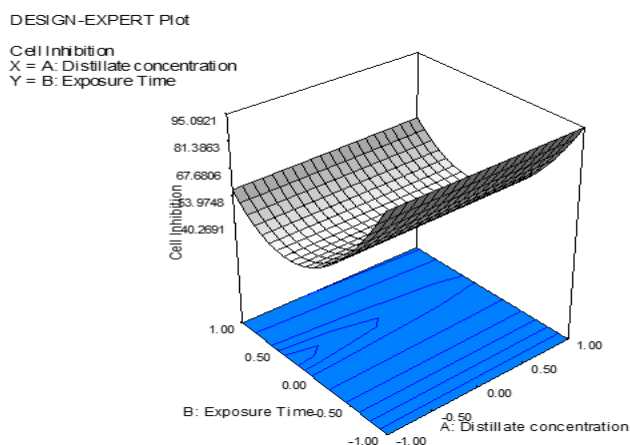
Fig. 4 Response surface for cell inhibition of distillates (MTT assay)
