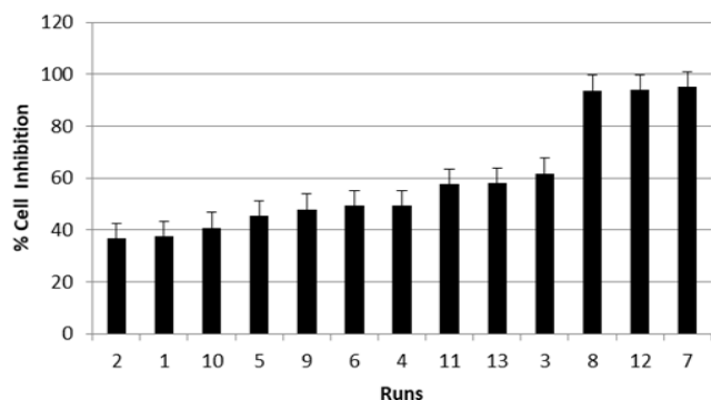
Fig. 3 . Cytotoxic effects of agarwood hydrosol against Calu-3 lung cancer tested using MTT assay. Samples were prepared based on Central Composite Design (CCD) with two factors (hydrosol amount and exposure duration) at three levels (high, medium, low). Samples (agarwood hydrosol) were added on already adherent cells to observe the ability of samples to kill the cells.. Untreated cells were used as negative control while 10% DMSO (v/v) was used as positive control.
