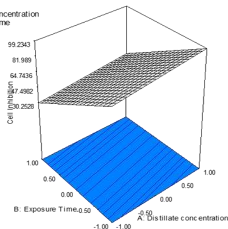
Fig. 2 Response surface plot showing the effects of hydrosol amount and exposure time on inhibition of cell attachment of Calu-3 cells as studied using Trypan blue dye attachment assay.
