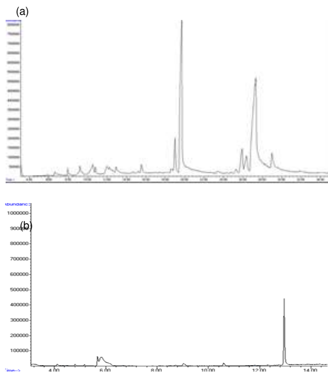
Fig. 5 Chromatograph of agarwood hydrosol using (a) GCMS and (b) HSPME-GCMS
