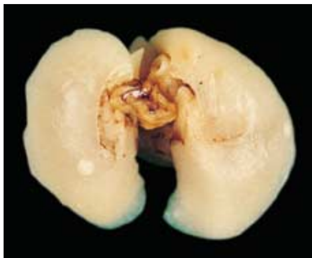
Fig. 2. Gross appearance of mouse lung with adenomas. Mouse was given a single subcutaneous injection of benzo(a)pyrene within 24 hr after birth and killed 9 weeks after birth.
