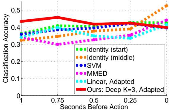
Figure 6: Performance vs \Delta : We plot performance on forecasting actions versus number of frames before the action starts. Our model (red) performs better when the time range is longer (left of plot). Note that, since our model takes days to train, we evaluate our model trained for one second, but evaluate on different time intervals. The baselines are trained for each time interval.
