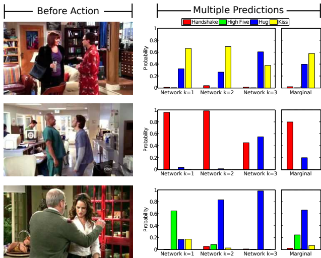
Figure 7: Multiple Predictions: Given an input frame (left), our model predicts multiple representations in the future that can each be classified into actions (middle). When the future is uncertain, each network can predict a different representation, allowing for multiple action forecasts. To obtain the most likely future action, we can marginalize the distributions from each network (right).
