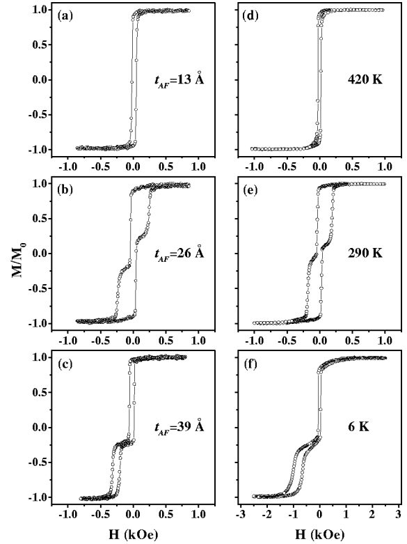
FIG. 1. Representative magnetization loops. Loops (a)–(c) were measured at 295 K for an IrMn layer thickness t_{AF} indicated, while loops (d)–(f) were taken at the temperatures indicated for a sample with t_{AF}=26 \text{ Å} . Curves (a), (b), (c), and (f) were measured by VSM, while curves (d) and (e) were measured by MOKE.
