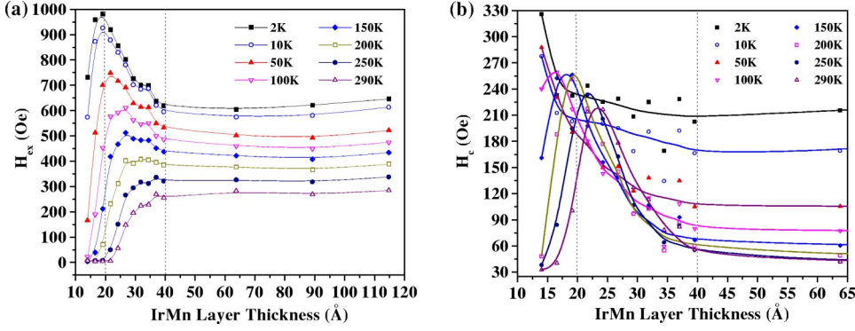
FIG. 3. IrMn thickness dependence of the exchange bias field H_{\text{ex}} (a) and coercivity H_c (b) for a number of temperatures. Lines between the points are a guide to the eye.
