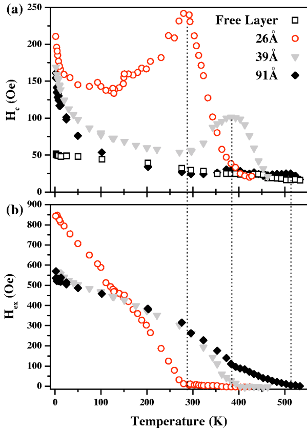
FIG. 2. Temperature dependence of the coercivity H_c (a) and exchange bias field H_{ex} (b) for selected IrMn thicknesses. The open square symbols represent the coercivity of the free Co layer within the spin valve. Samples were initially field cooled in 0.4 T field to 2 K before commencing measurements. The vertical dashed lines indicate the blocking temperatures of the three samples.
