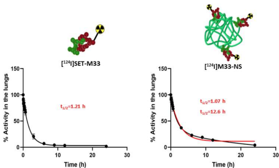
Figure 5 Pharmacokinetics. Decay curves for [^{124}\text{I}]\text{SET-M33} and [^{124}\text{I}]\text{M33-NS} , obtained from the in vivo quantification results. Half-life values are shown in red.
