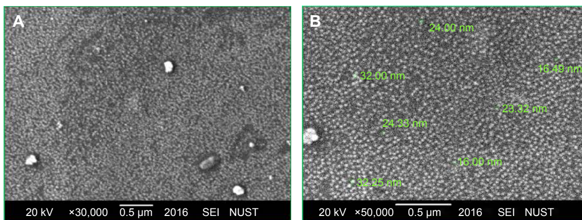
Figure 4 SEM images of green synthesized CeO 2 NPs. (A) Magnification ×30,000; (B) Magnification ×50,000.
