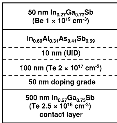
FIG. 2. Layer structure indicating the composition, doping and thickness of a diode. The 10 nm UID layer was included to minimize any possible Te segregation from the heavily doped \text{In}_{0.69}\text{Al}_{0.31}\text{As}_{0.41}\text{Sb}_{0.59} into the p^+ \text{In}_{0.27}\text{Ga}_{0.73}\text{Sb} .
