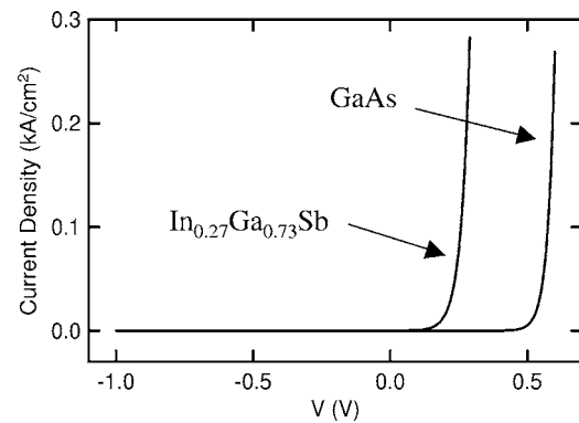
FIG. 4. Comparison of the bias dependence of the dc density for an \text{In}_{0.27}\text{Ga}_{0.73}\text{Sb}/\text{In}_{0.69}\text{Al}_{0.31}\text{As}_{0.41}\text{Sb}_{0.59} heterojunction pn diode and a GaAs Schottky diode. The heterojunction reaches a given current density at a lower dc bias than the GaAs Schottky.
