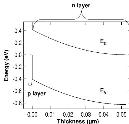
FIG. 1. Energy band diagram to emphasize the very thin p layer, the 0.5 eV bandgap of the p layer, and the large valence band offset.
