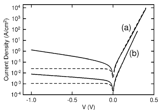
FIG. 3. I - V for two different diodes. (a) has the layer structure shown in Fig. 2 and (b) has a lower doped, thicker n layer without the 10 nm UID part.
