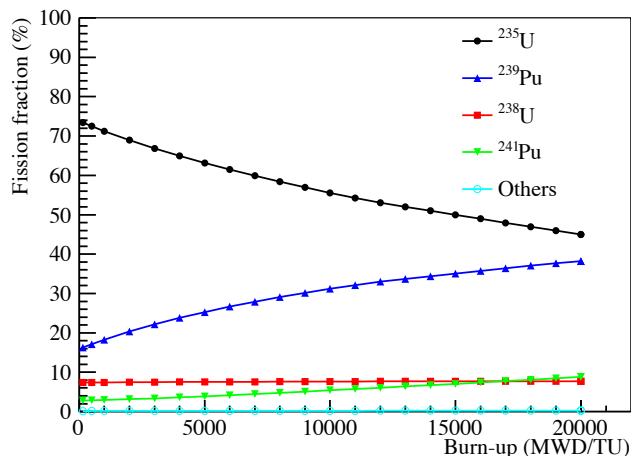
Fig. 1. Fission fractions of isotopes as a function of burn-up from a simulation of a reactor core at the Daya Bay nuclear power plant. Other isotopes contribute less than 0.3% in total.
