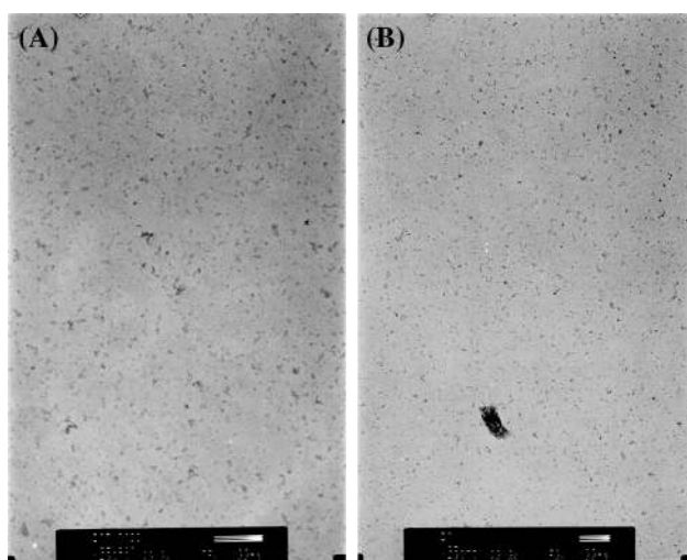
Fig. 6 TEM images of the CuO nanoparticles synthesized using extract of G. herba where a the scale bar is 100 \mu\text{m} and b the scale bar is 200 \mu\text{m}
