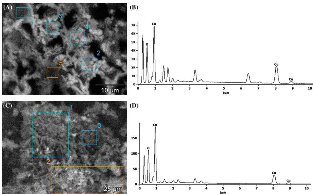
Fig. 5 SEM images of the CuO nanoparticles using extract of G. herba where a the scale bar is 10 \mu\text{m} and c the scale bar is 25 \mu\text{m} and EDS profiles ( b , d )
