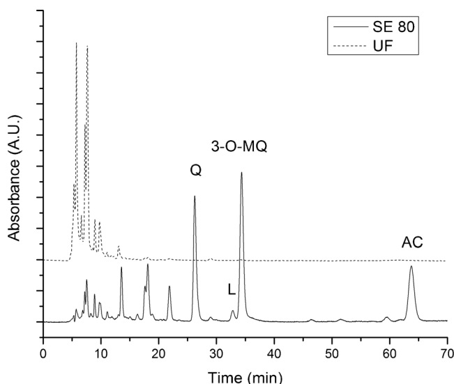
Fig. 2. Chromatogram of extract (full line; 50 \times diluted) and ultrafiltrated NEE (dotted line). It can be seen that important flavonoids (quercetin (Q), luteolin (L), 3- O -methylquercetin and achyrobichalcone (AC)) were completely incorporated to the nanoemulsion structure in the assayed conditions
