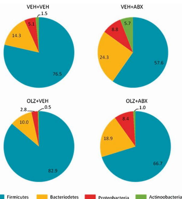
Figure 1. Effect of olanzapine (OLZ) coadministered with vehicle (VEH) or an antibiotic cocktail (ABX) on the faecal microbiota of female rats. N = 6 .
