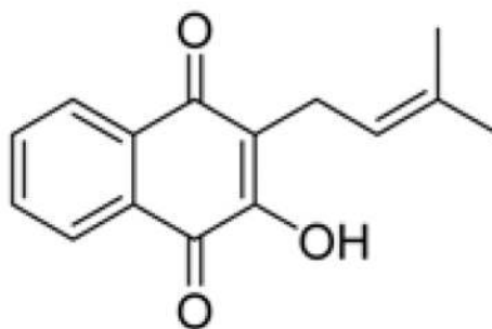
Lapachol
