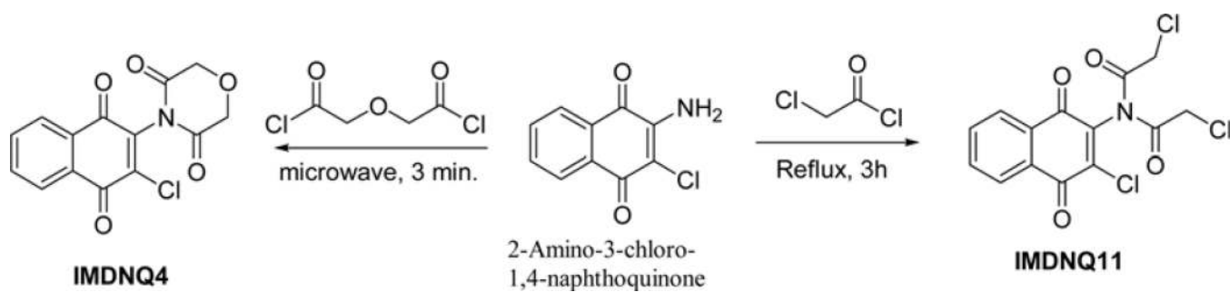
Scheme 1.
