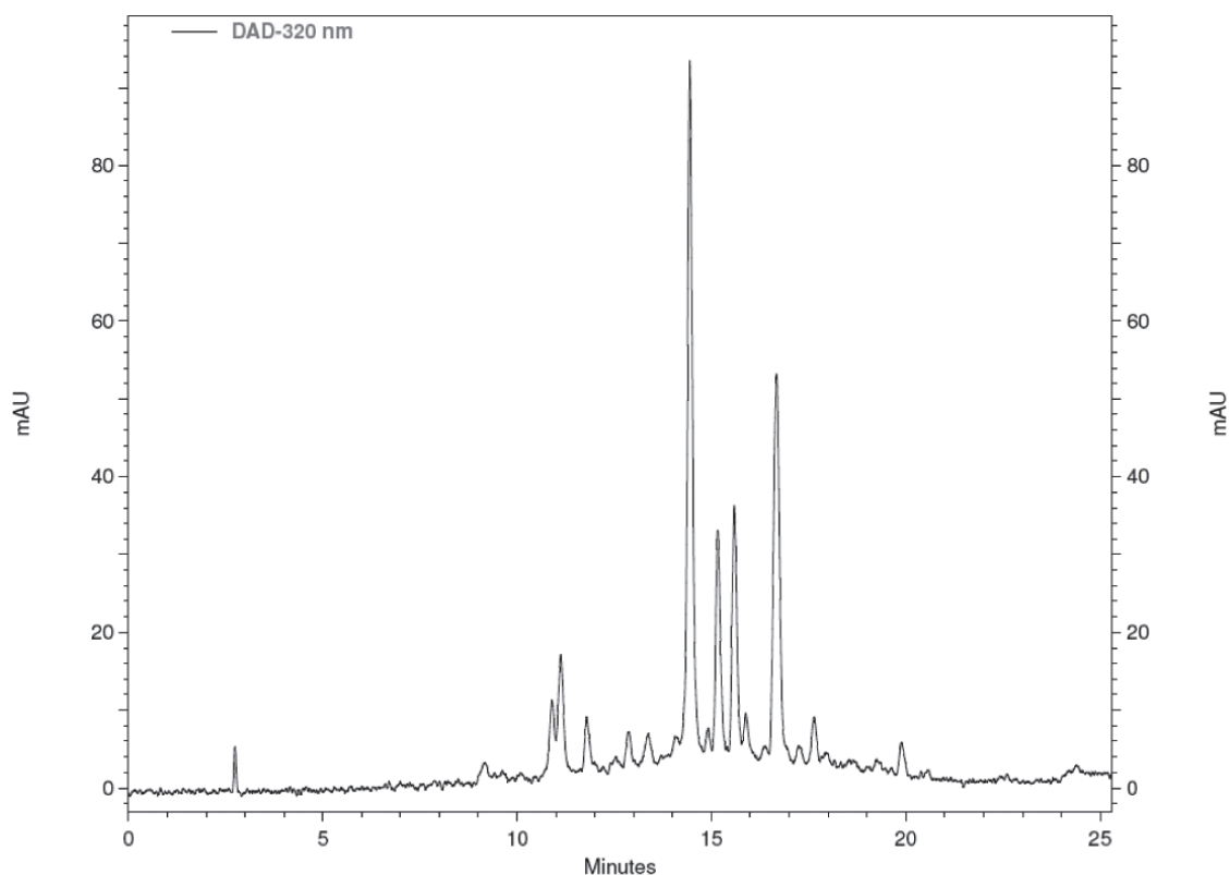
Figure 4: HPLC-DAD phenolic profile for ES-EtOH recorded at 320 nm.
