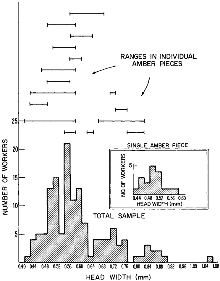
Fig. 8. Azteca alpha workers: size range between and within series found within individual amber pieces and hence assumed to belong to the same colony. The larger frequency curve ( bottom in figure ) includes all of the 141 workers measured. The smaller frequency curve ( enclosed in rectangle ) includes the measurable workers from one of the most populous pieces. The series of horizontal bars ( uppermost in figure ) depict the ranges within single amber pieces. The samples originate variously from Carlos Diaz, La Bucara, Las Bocas del Licey, Llaroa, Los Cacaos, Palo Quemado, and still other, unknown mine sites within the Dominican Republic.
