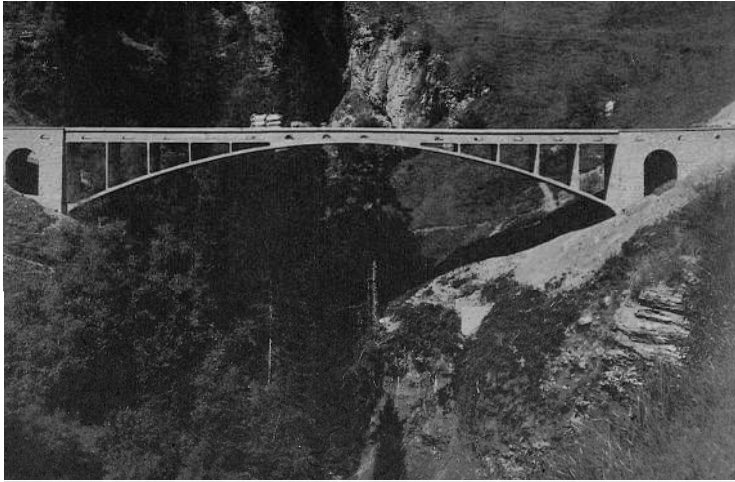
Left: Robert Maillart. Valtschielbach Bridge, Donath, Switzerland, 1925.
