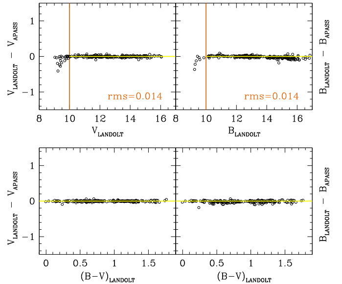
Figure 5. Comparison between the source B , V data of the Landolt (2009) equatorial standards and the corresponding APASS values. The vertical line marks where saturation of brighter stars sets in (because of APASS fixed exposure times) under excellent seeing conditions. Saturated stars from top panels are not plotted on lower panels.
