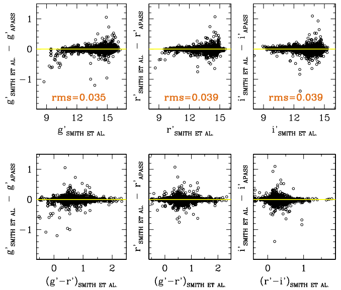
Figure 7. Comparison between the g' , r' , i' data of 2988 secondary Sloan standards provided by Smith et al. (2002) and the corresponding APASS values. (A color version of this figure is available in the online journal.)
