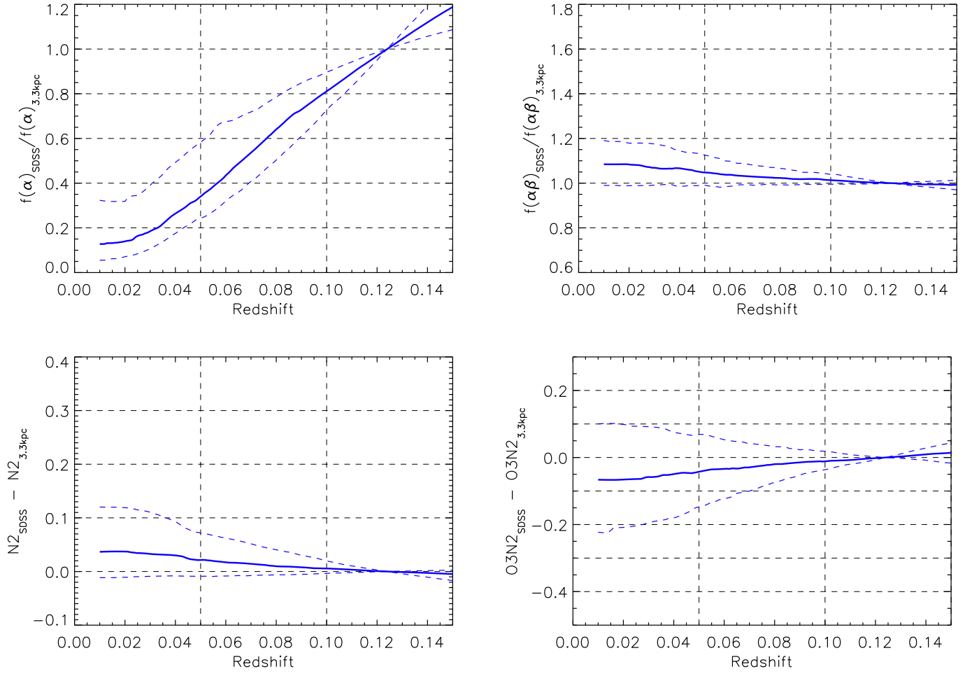
Figure 16. Ratio of the H \alpha flux (top left), H \alpha /H \beta (top right), N2 (bottom left), and O3N2 (bottom right) contained in the SDSS aperture at different redshifts to the corresponding values within a circular aperture of 3.3 kpc diameter as a function of redshift for the (96) CALIFA spirals whose 3.3 kpc diameter aperture is completely covered by PMAS/PPAK. Lower dashed, solid, and upper dashed lines correspond to 15.86%, 50%, and 84.14% of the distributions.
