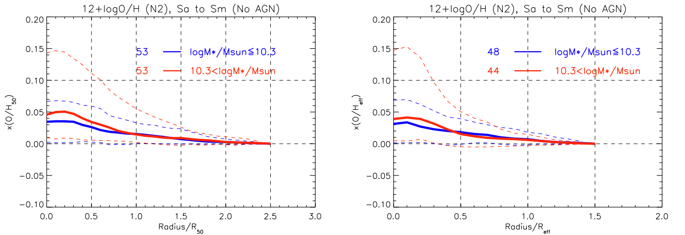
Figure 21. Left: x(OH_{50}) for two different stellar mass bins, estimated with N2 (M13). Solid lines correspond to median values. Dashed lines contain 68.2% of the distribution. Galaxies with \log M^*/M_{\odot} \leq 10.3 and \log M^*/M_{\odot} > 10.3 are represented in blue and red, respectively. Right: same as left for x(OH_{eff}) .
