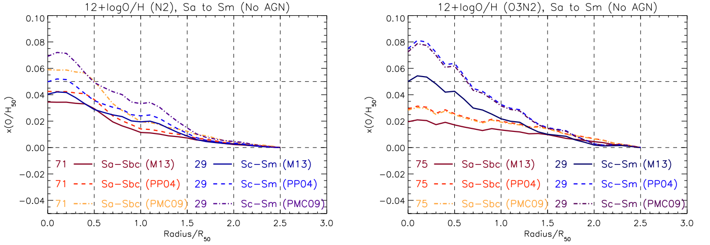
Figure 19. Left: x(O/H_{50}) for two different morphological type bins, and the three empirical calibrations of N2: PP04, PMC09, and M13. Right: x(O/H_{50}) for two different morphological type bins, and the three empirical calibrations of O3N2: PP04, PMC09, and M13.
