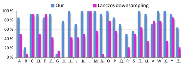
Figure 7: Character recognition: Standard filtering vs. Ours. Dark horizontal lines indicate significant statistical difference.
