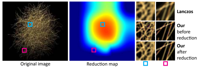
Figure 5: Flickering reduction. Left: Original high resolution image. Center: Reduction map. Right: Outcome of Lanczos filtering, as well as our approach before and after flickering reduction for the marked regions. Note that in the regions of strong temporal contrast reduction an improvement over Lanczos filtering is visible. Similar to Fig. 4, images for our approach are simulations of perceived images assuming motion and perfect eye tracking.
