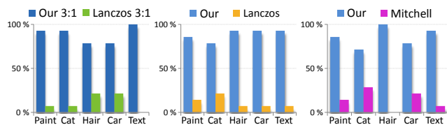
Figure 6: Our method against Lanczos in 3:1 scale (left) and original scale (middle) as well as Mitchell-Netravali (right).
