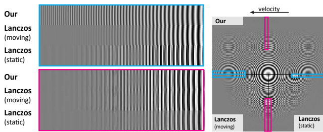
Figure 4: Our method vs. Lanczos. Our method uses image motion to improve the perceived resolution along this movement direction by showing 3 subimages on a rapid display. While we rely on a frame optimization, moving Lanczos resampling derives subimages by filtering the translated original image. The eye integration is computed by blending the subimages, assuming perfect tracking.
