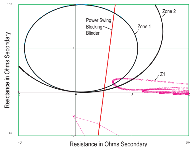
Fig. 19. Impedance Plan Plot of High-Load Power Swing Blocking Scheme
