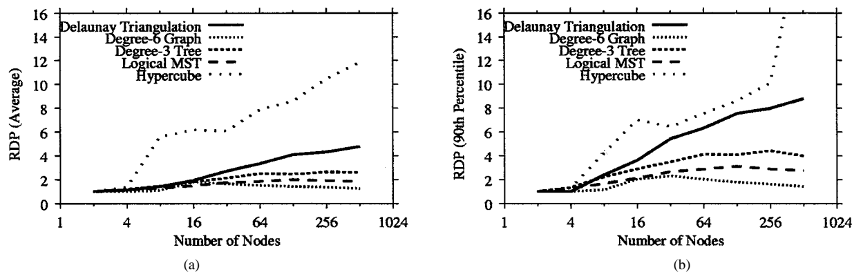
Fig. 7. RDP. (a) Average. (b) 90th percentile.
