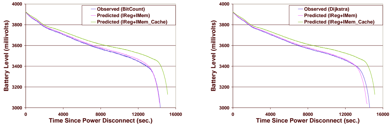
Integer Benchmarks BitCount (left) and Dijkstra (right)
