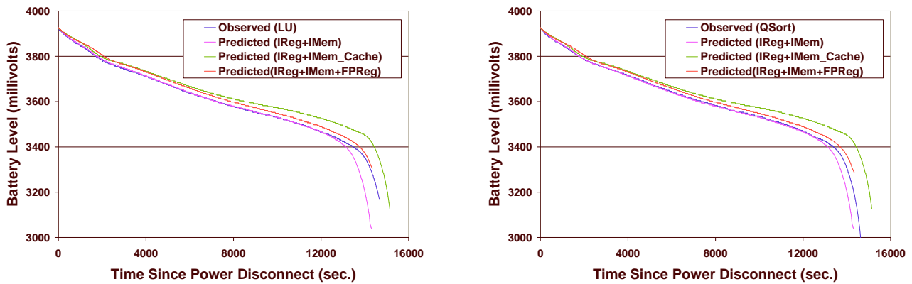
Floating Point Benchmarks LU (left) and QSort (right)
