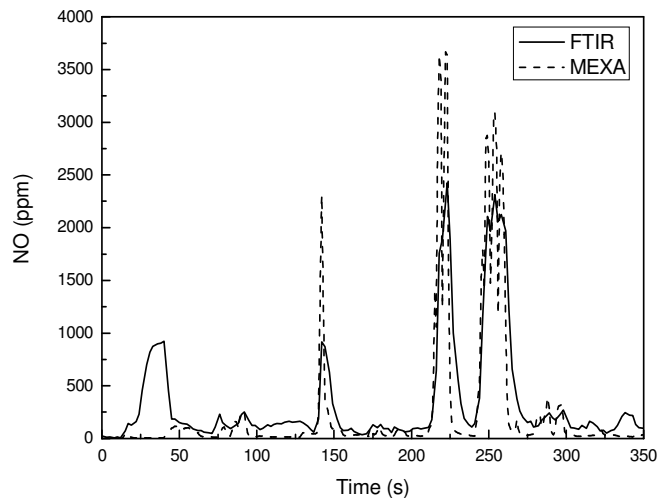
Figure 10: FTIR vs. MEXA for NO x
