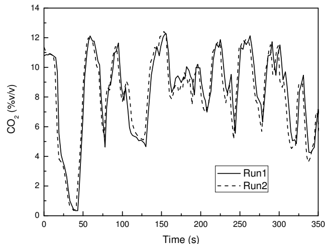
Figure 12: FTIR CO 2 repeatability
