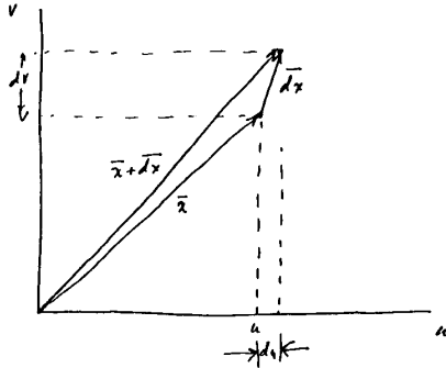
Fig. 2. The enclosed area is \frac{1}{2} |\det \begin{bmatrix} u & v \\ v & du/dv \end{bmatrix}| .
