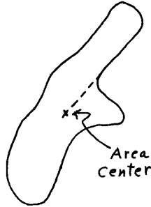
Fig. 3. Rotating counterclockwise about the center of gravity, a discontinuity occurs in the parameterization if the boundary has a finite arc which aligns with the radius.
