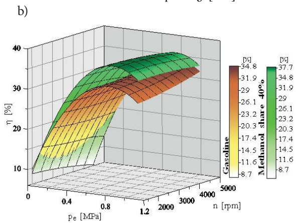
Fig. 8. Comparison of overall efficiency of 1100 MPI Fiat engine in case of feeding with petrol or two fuels at various shares of methanol
