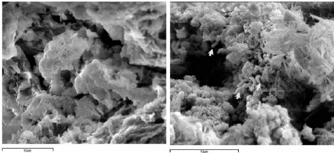
FIGURE 3 | Scanning electron microscopy (SEM) observations of Carbogel without (left) and with (right) D. vulgaris subsp. vulgaris ATCC 29579 cells (Source: Cappitelli et al., 2006).
