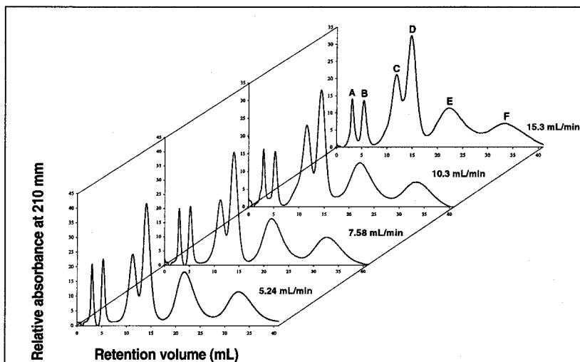
Figure 4. The effect of flow rate on the organic acid isocratic separation on the QA CIM monolithic column of 12-mm length: pyruvic acid (0.03-g/L sample), A; malic acid (0.5-g/L sample), B; \alpha -ketoglutaric acid (0.2-g/L sample), C; fumaric acid (0.007-g/L sample), D; citric acid (2-g/L sample), E; and isocitric acid (2-g/L sample), F. Conditions: 130mM NaCl in 20mM phosphate buffer mobile phase; 5.24-, 7.58-, 10.3-, and 15.3-mL/min flow rates.
