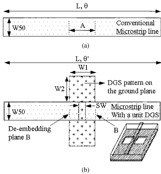
Fig. 1. (a) Conventional microstrip line; (b) microstrip line with a unit DGS pattern and the same length ( W50 = 1.4 mm, SW = 0.5 mm, W1 = W2 = 2 mm). The substrate with 20 mils of thickness, 2.6 of dielectric constant, and 18 \mu\text{m} of metal thickness is adopted in this work.
