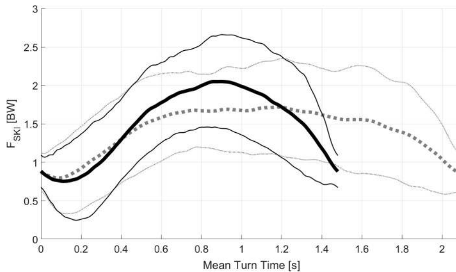
FIGURE 3 | Turn cycle characteristics for ground reaction force ( F_{SKI} ) for Giant slalom in black and Super-G in gray as a function of mean turn cycle time. Instantaneous mean in solid line, Standard deviations in thin line.
