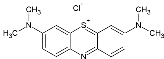
Figure 15. Molecular structure of Methylene Blue.
