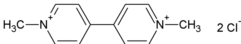
Figure 10. Molecular structure of Methyl Viologen.
