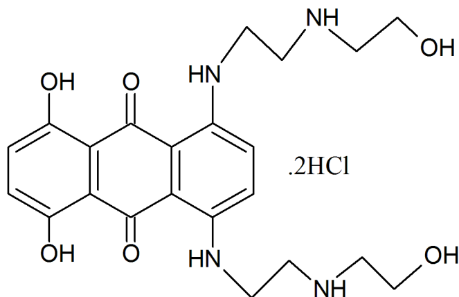
Figure 8. Molecular structure of Mitoxantrone.
