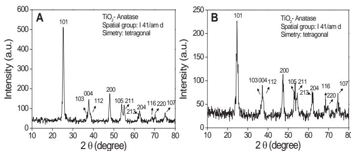
Figure 13. X-ray diffractograms of \text{TiO}_2 synthesized by the molten salt method: (A) in \text{NaNO}_3 and (B) in \text{KNO}_3 .
