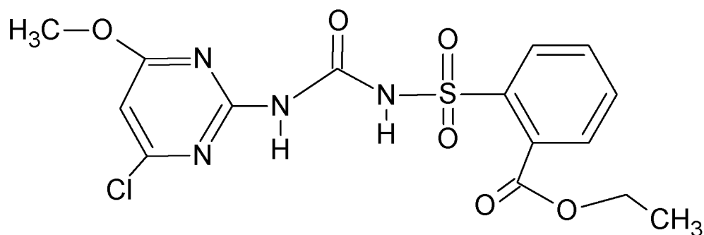
Figure 6. Molecular structure of Chlorimurom-ethyl (CE).
