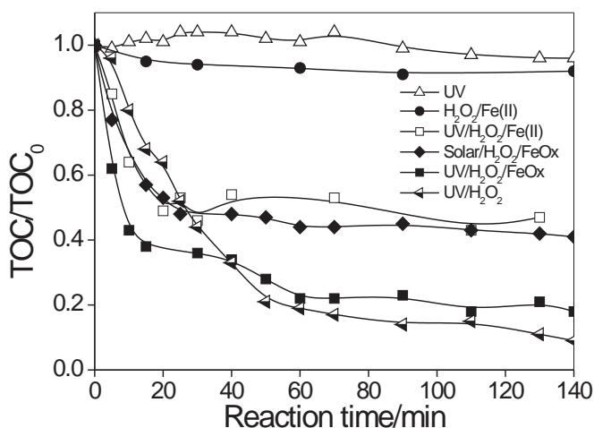
Figure 9. Comparison of the mineralization of aqueous MTX solutions (0.077 mmol L -1 ) by different AOP (0.54 mmol L -1 iron source and 18.8 mmol L -1 H 2 O 2 , when present).
