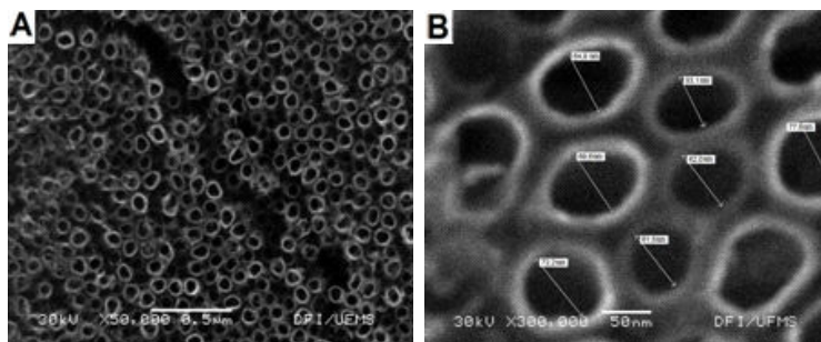
Figure 17. Scanning electron micrographs of TiO 2 nanotubes prepared on a Ti film in 0.15 mol L -1 NH 4 F in glycerol (10% H 2 O) at a potential of 20 V. (A) TiO 2 nanotubes, (B) diameters of the nanotubes.
