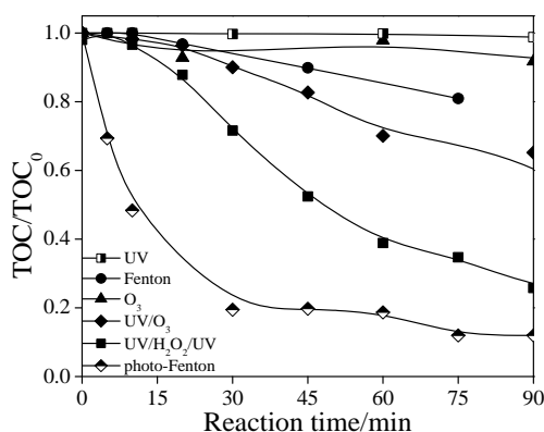
Figure 7. Comparison of the efficiencies of mineralization of a commercial formulation of CE in aqueous solution by the different AOP. [CE]_0 = 0.060 \text{ mmol L}^{-1} ; [TOC]_0 = 65 \text{ mg L}^{-1} ; when present, [Fe^{2+}] = 0.2 \text{ mmol L}^{-1} , [H_2O_2] = 68.4 \text{ mmol L}^{-1} and [O_3] = 25 \text{ mg mL}^{-1} .
