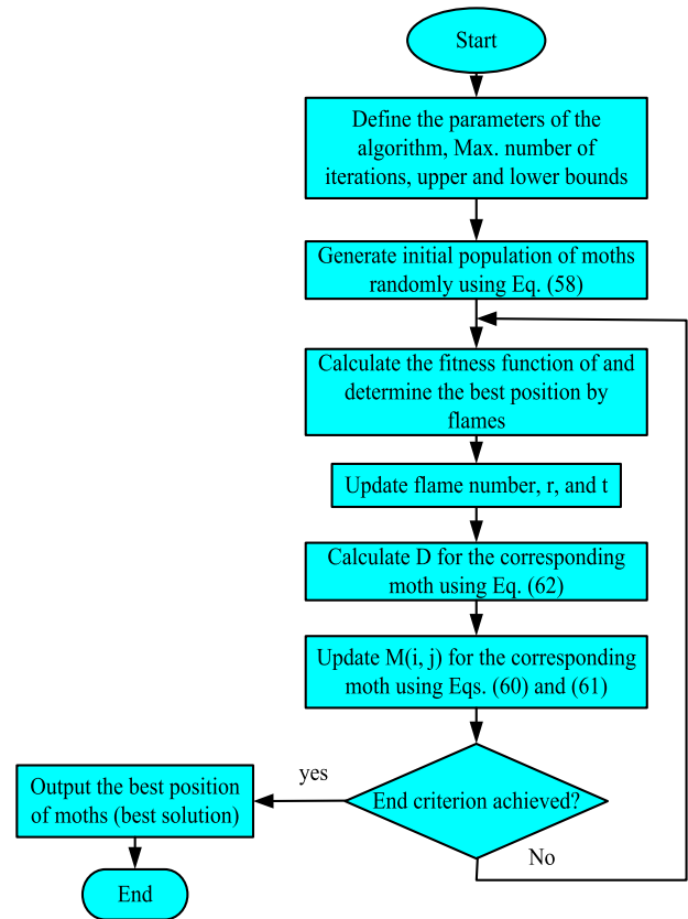
FIGURE 9. Flow chart of the MFO optimization algorithm.
