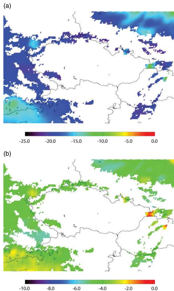
Figure 2. Images of 31 May 2008 nowcast time period 1100 UTC (a) 6.2-7.3 \mu\text{m} channel difference and (b) tri-channel [(8.7-10.8)-(10.8-12.0)] \mu\text{m} difference.
