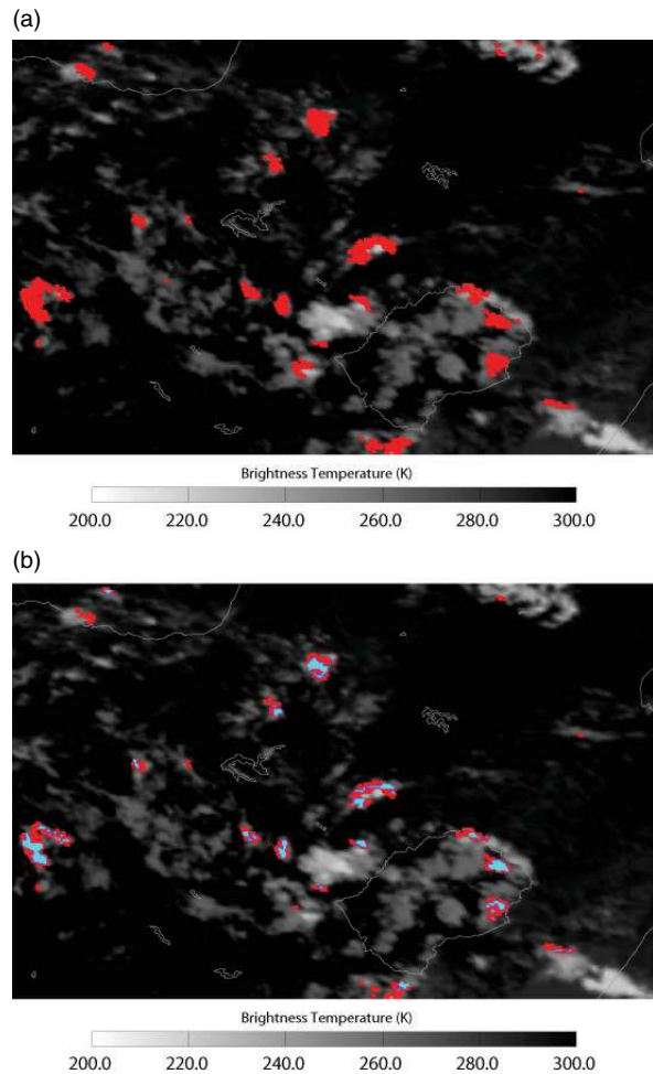
Figure 8. The CI nowcast product overlaid on 10.8 \mu\text{m} brightness temperatures for 7 February 2008 at 1030 UTC over South Africa for the (a) Mecikalski and Bedka (2006) method and (b) using MSG specific interest fields.
