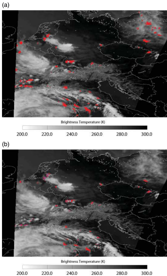
Figure 7. CI nowcast overlaid on 10.8 \mu\text{m} brightness temperatures for 31 May 2008 at 1100 UTC over central Europe from the (a) Mecikalski and Bedka (2006) method and (b) using MSG specific interest fields.
