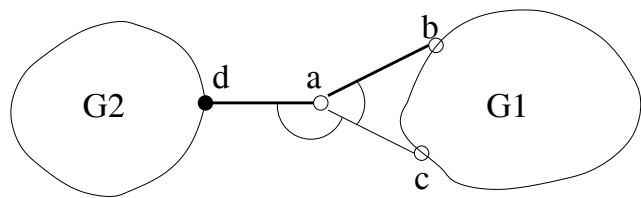
Fig. 11. An example where the TP-algorithm is not irreducible. Turn (c, a, d) is prohibited while it could be permitted. The special node and special links are marked in bold.
