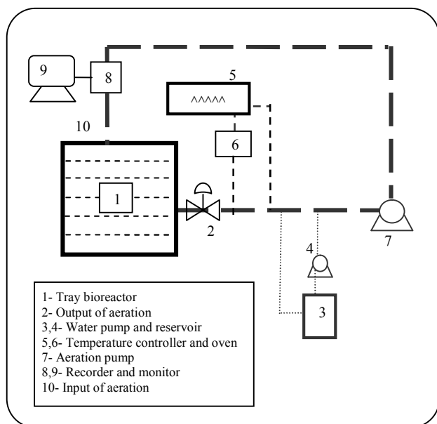
Fig. 1: Schematic diagram of experimental apparatus for solid state fermentation of sugarcane in a constant level of moisture in gas phase (not to scale).
