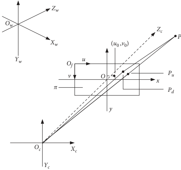
FIGURE 1: Pin-hole imaging principle diagram.
