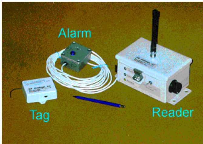
Figure 4. IDI's prototype collision avoidance system
