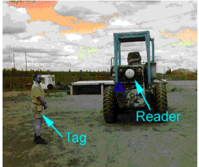
Figure 1. Test configuration of UHF RFID system.
