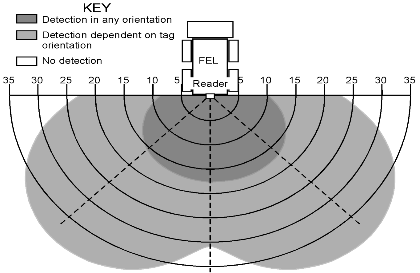
Figure 2. Test results of UHF RFID system.
