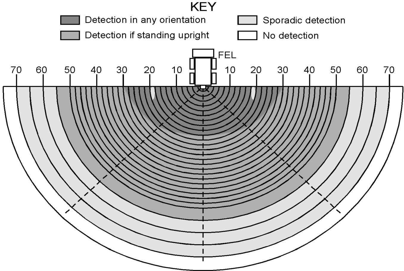
Figure 5. Test results of IDI system.
