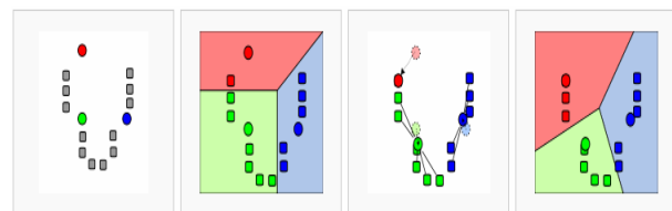
1) k initial "means" (in this case k=3) are randomly generated within the data domain (shown in color). 2) k clusters are created by associating every observation with the nearest mean. The partitions here represent the Voronoi diagram generated by the means. 3) The centroid of each of the k clusters becomes the new mean. 4) Steps 2 and 3 are repeated until convergence has been reached.
