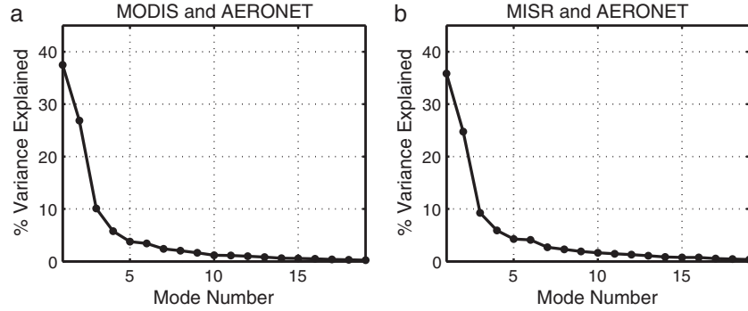
Figure 2. Variance explained by the maximum covariance analysis (MCA) modes for (a) Moderate Resolution Imaging SpectroRadiometer (MODIS) and AERONET and (b) Multi-angle Imaging SpectroRadiometer (MISR) and AERONET, decomposed using the full data sets.
