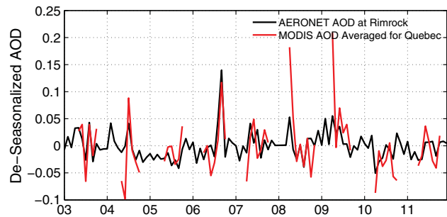
Figure 10. Time series of AERONET AOD at Rimrock and MODIS AOD averaged over the Quebec region that is correlated with Rimrock. The lack of sampling of MODIS data during winter and coincident agreements during some summer months results in the spurious correlation between these two remote locations.
