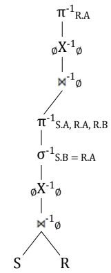
Figure 13. RRA Tree for Exists Query, Case 2.
