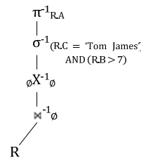
Figure 7. RRA Tree for Group-by Query, Case 1.
