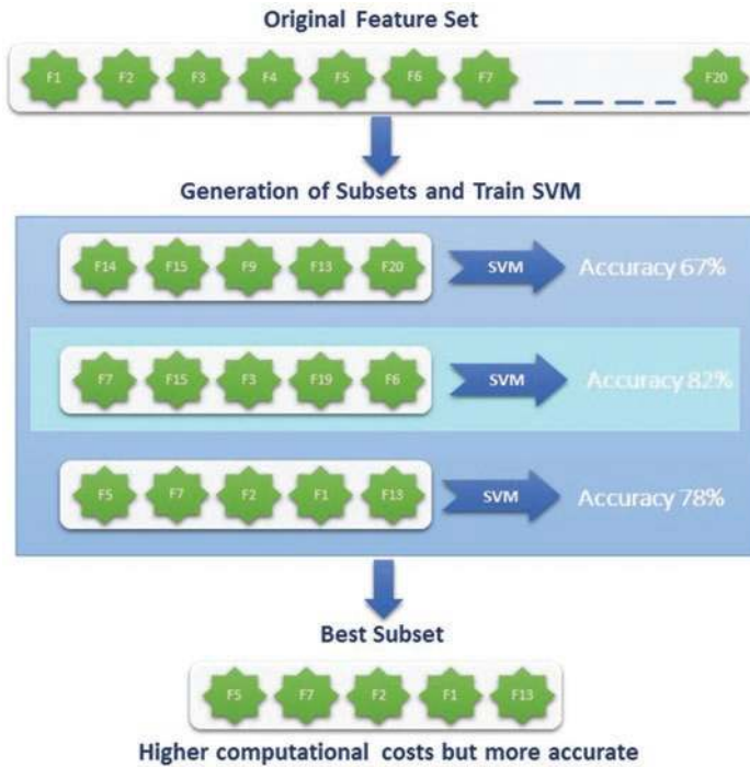
Fig. 9 Wrappers & classification accuracy
