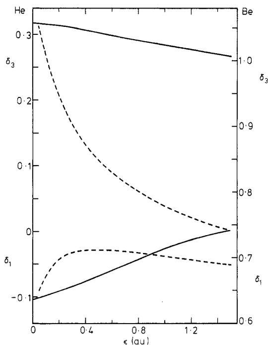
Figure 1. Elastic p-wave phaseshifts for e\text{-He}^+ and e\text{-Be}^+ scattering plotted against continuum electron energy \epsilon . The full curves give RRPAs values for e\text{-He}^+ scattering; \delta_1 refers to the singlet phaseshift and \delta_3 refers to the triplet phaseshift. The broken curves give RRPAs values for e\text{-Be}^+ scattering. The right-hand scale refers to Be. For all cases the Coulomb phaseshift has been removed.
