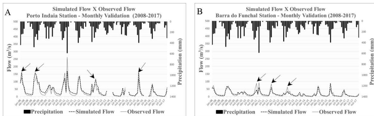
Figure 4. Flow simulation in validation – Porto Indaia Station (a) and Barra do Funchal Station (b).
