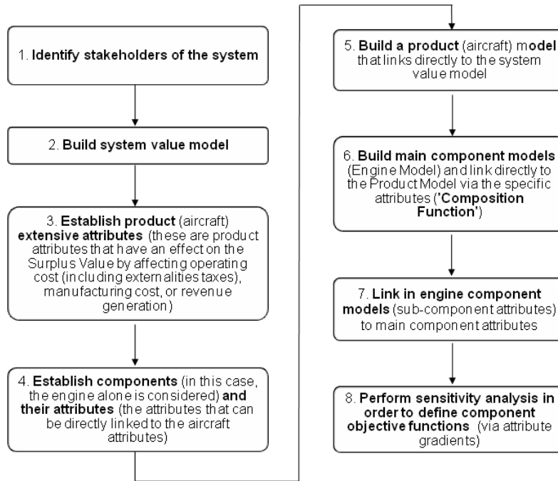
Figure 6: Generalized VDD modeling process steps
