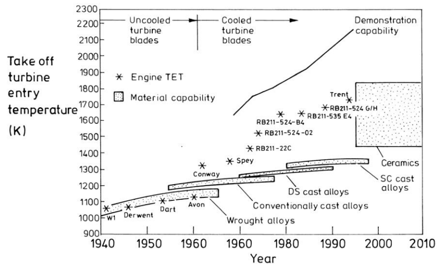
Figure 12: Turbine entry temperature for Rolls-Royce engines since 1940
