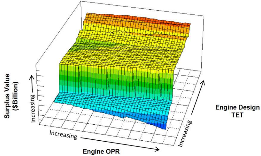
Figure 14: Sample results - Surplus Value vs. engine OPR and engine design TET
