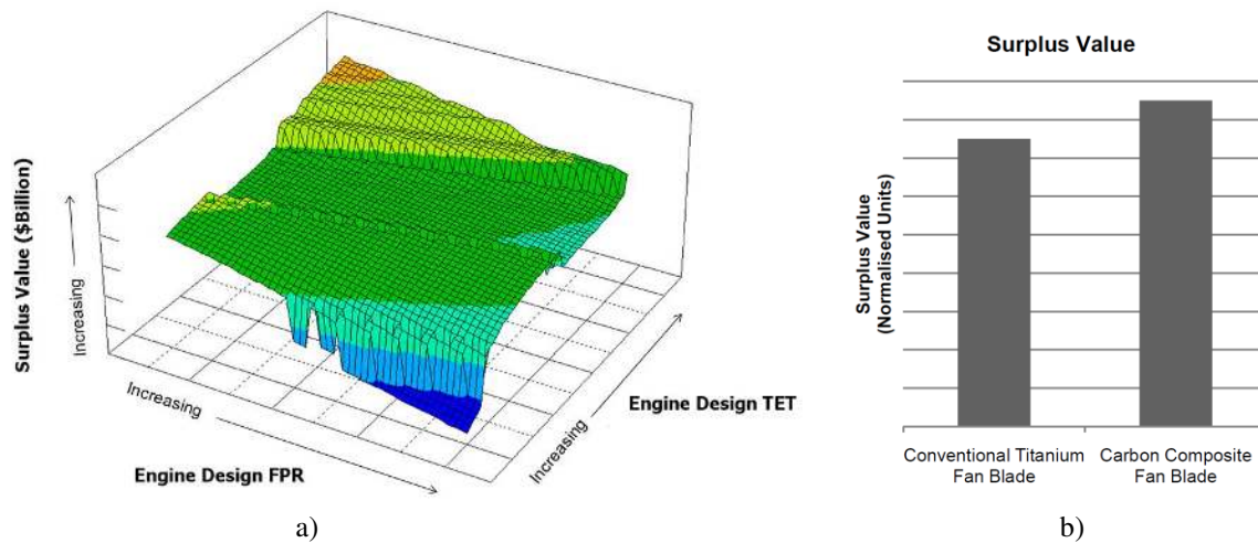
Figure 17: Sample results, a) surface plot of Surplus Value against FPR and TET, b) Surplus Value difference between Titanium and Composite fan blades
