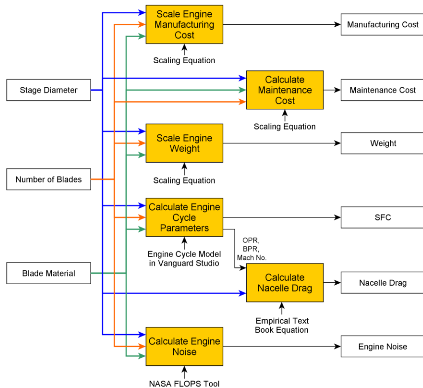
Figure 16: Engine and component attributes map for fan blade material study
