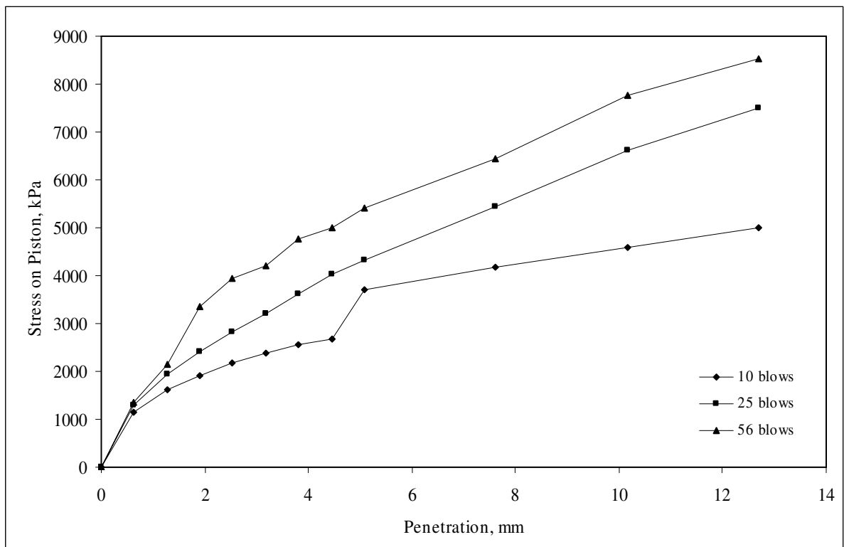
Figure 45: Penetration vs. Stress, CBR Test, 2:1 Mix Ratio, 56 Days
