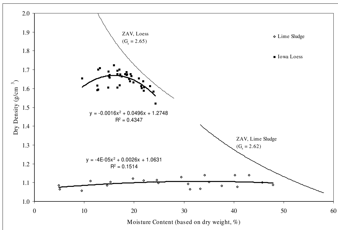
Figure 24: Moisture-Density Relationship.
