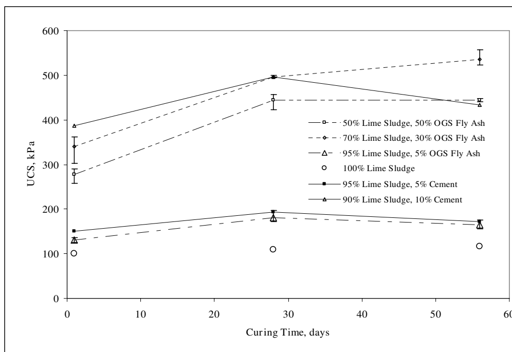
Figure 16: Effect of Curing Time on Lime Sludge and Cement/Fly Ash Mixtures
