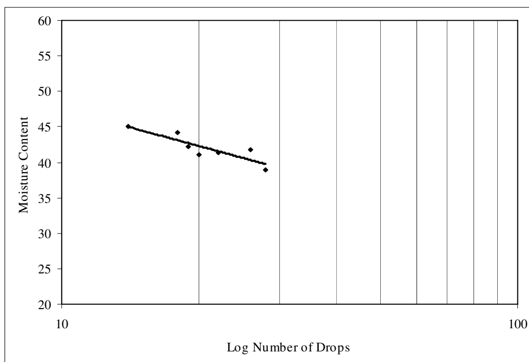
Figure 23: Liquid Limit Data for Lime Sludge
