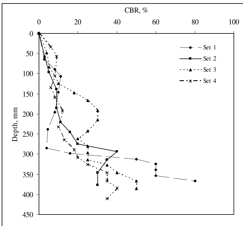
Figure 62: CBR as a Function of Depth for Test Embankment, April 2005
