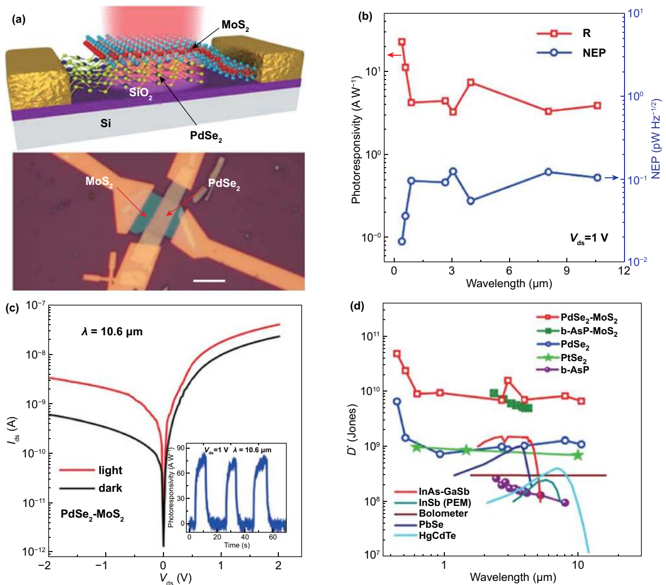
Fig. 22 PdSe 2 /MoS 2 van der Waals heterostructure-based photodetector. a Scheme of the PdSe 2 /MoS 2 photodetector (top) and optical micrograph of the corresponding device (bottom), where the scale bar is 5 μm. b Wavelength dependence of photoresponsivity (red) and noise equivalent power (blue) of the PdSe 2 /MoS 2 photodetector at V DS = 1 V. NEP denotes noise equivalent power. c Drain current of heterostructure-based device under illumination and in the dark. The inset shows the current profile against time with periodic light illumination and dark state. d Wavelength-dependent detectivity of different 2D materials and some infrared materials at room temperature. Reprinted with permission from Ref. [54]. Copyright 2019, American Chemistry Society
