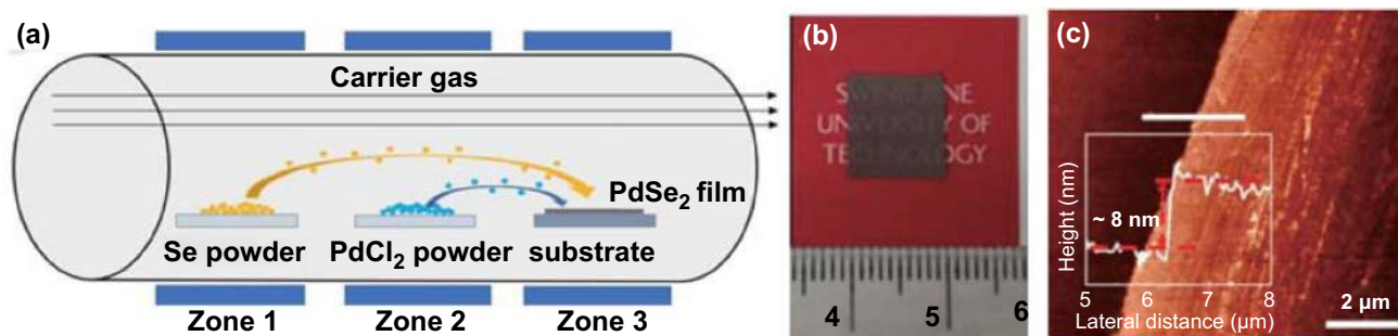
Fig. 12 a Schematic of PdSe 2 synthesis process using CVD method. b, c Photograph and AFM height profile of a prepared multilayer PdSe 2 film. Reprinted with permission from Ref. [60]. Copyright 2020, American Chemical Society
